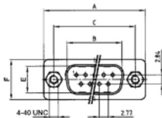
Plug connector
