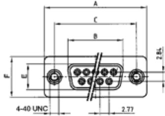
Socket connector
