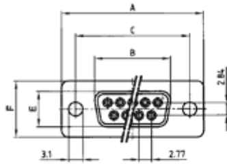
Socket connector
