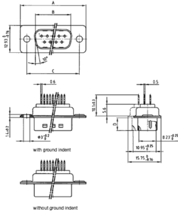
Plug connector
