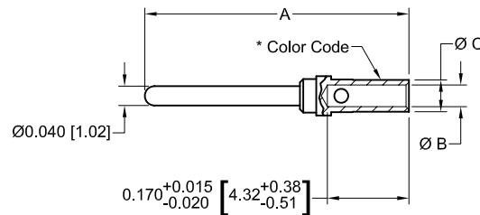
MALE CONTACT
